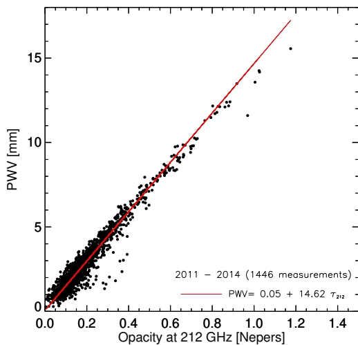
Figure 4. Correlation between the atmospheric opacity at 212 GHz and the precipitable water vapor (PWV) for the period of January 2011 to July 2014, at "El Leoncito" site.
