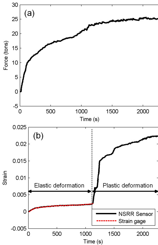
Figure 3. Results of the simply supported beam experiment: a) Applied force versus time, b) The change of strain read from the wireless sensing system compared to strain gages (for elastic region only).
