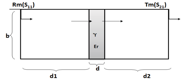
Figure 2 Theoretical modeling of the Transmission device
