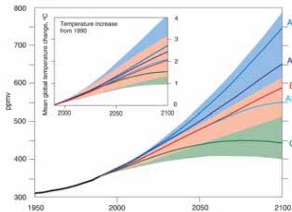
Fig. 1.2.8. Atmospheric CO 2 concentrations, in ppmv, historical development from 1950 to 1990 and in scenarios to 2100. The insert shows global mean temperature change compared with 1990 in degrees Celsius. The (substantial) model uncertainties are also indicated. 16
