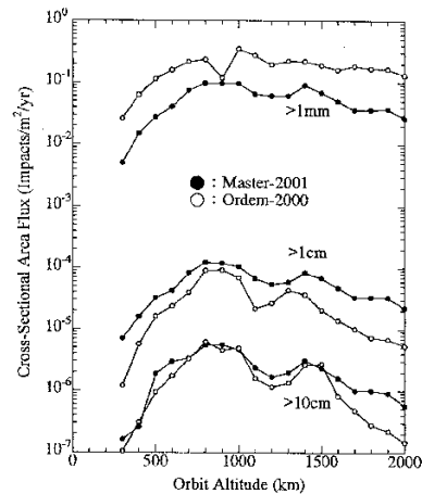
Fig. 2.3.3 Space debris flux below 2000 km (Orbit inclination 0 degree, AD2030)
