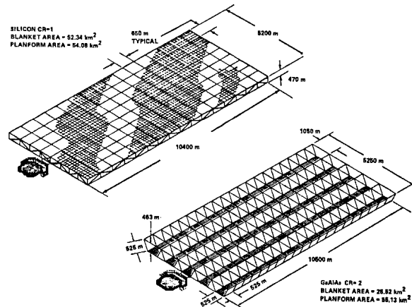
Fig. 2.4.2 NASA-DOE SPS Reference Model
