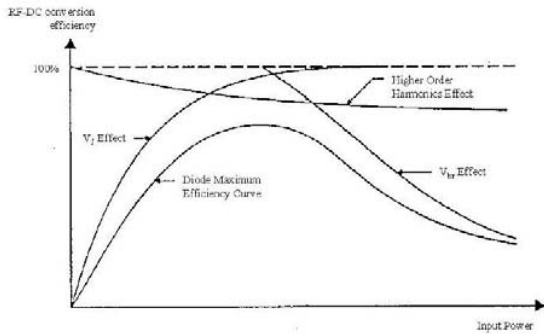
Fig. 2.3.17 Typical rectenna RF-DC conversion efficiency 68
