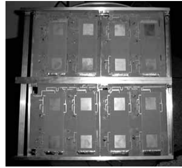
Fig. 3.2.3 The 2x2 AIA panel array. 15
