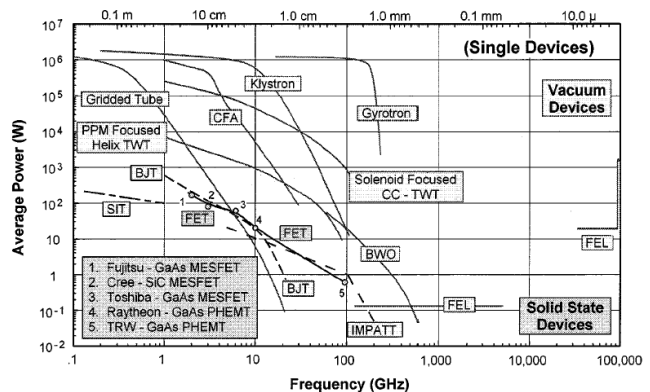
Fig. 3.2.1 Average RF output power versus frequency for various electronic devices 10 and semiconductors. 12
