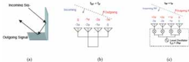
Fig. 2.3.15. (a) Two-sided corner reflector. (b) Van Atta Array. (c) Phase-conjugating array. (Sung et al., http://hac.hawaii.edu/tcwct03/papers/s16p03.pdf ) 55
