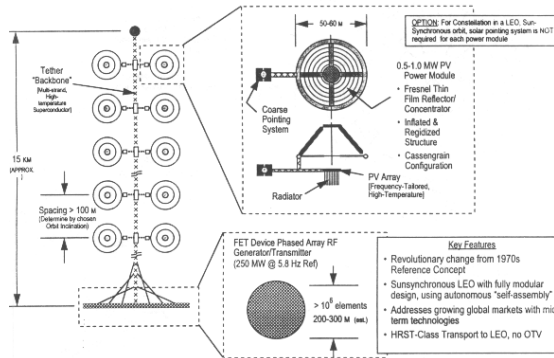
Fig. 2.4.4 The "Sun Tower" SSP Concept (MEO constellation)
