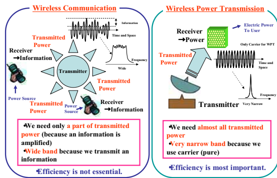
Fig. 3.6.1 Difference between wireless communication and wireless power transmission. ©RISH, Kyoto University
