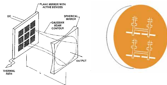
(a) Cavity type! ! ! ! ! (b) Array type
