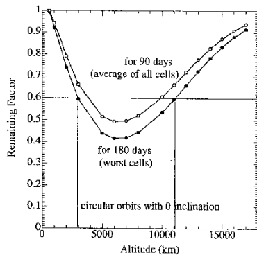
Fig. 2.3.2 Deterioration of efficiency of the solar cells during 6 months Altitude vs. Remaining Factor -
