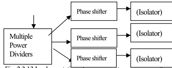
Fig. 2.3.13 Implementation of microwave transmission with a high power microwave oscillator and phase-shifters for high precision control of microwave beam direction to large angles without grating lobes 36
