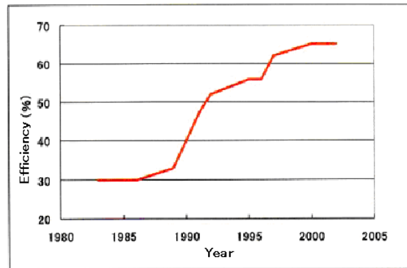
Fig.2.3.12 Trend of Efficiency of TWTA 44
