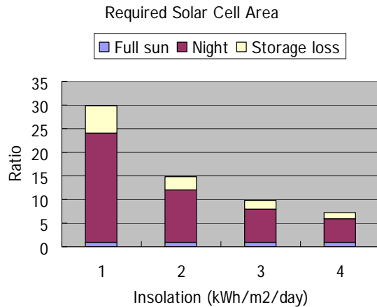
Fig. 2.1.4 Required solar cell area when a terrestrial solar power system is used as base load.
