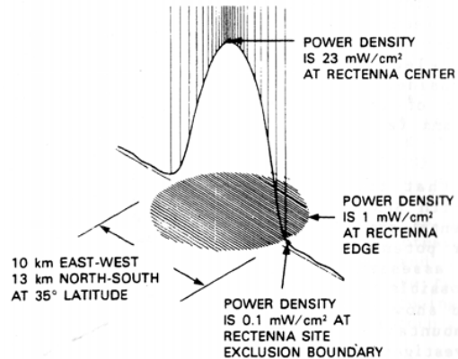
Fig. 2.4.3 Power density distribution at rectenna site on the ground.
