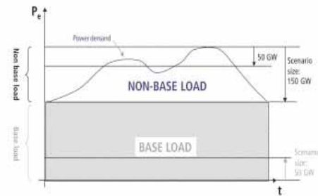
Fig. 2.4.15 Definition of base- and peak-load (non-baseload) power as used for the present assessment.
