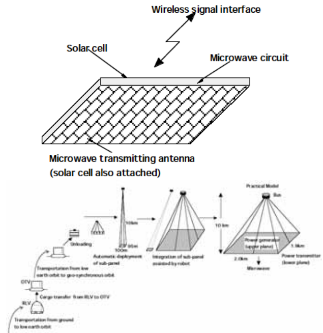
Fig. 2.4.13 Overall construction scenario
