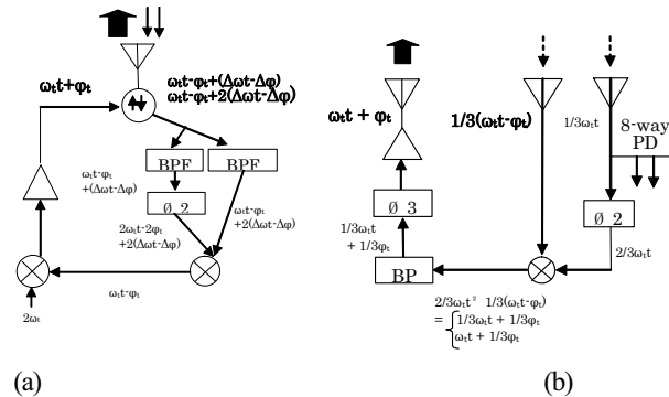
Fig. 2.3.16 Phase conjugate circuit developed in Kyoto University © RISH, Kyoto University
