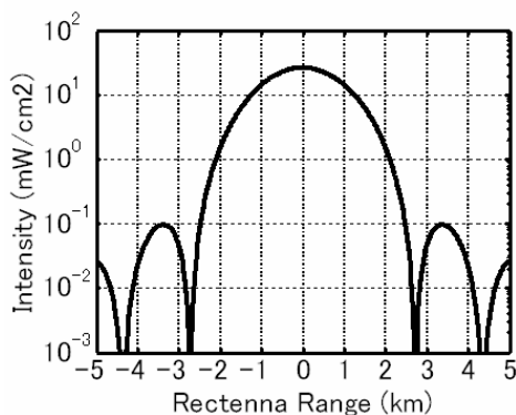
Fig. 2.2.1 Typical power density at a rectenna site (1km \phi TX antenna with 10dB Gaussian power distribution)
