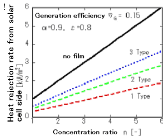
Figure 2.3.10 Relation between sunlight concentration ratio and heat rejection rate (with spectral filter attached) 33
