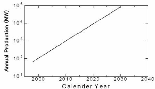
Fig. 2.3.5 Prediction of Solar Cell Production (From NEDO Website)
