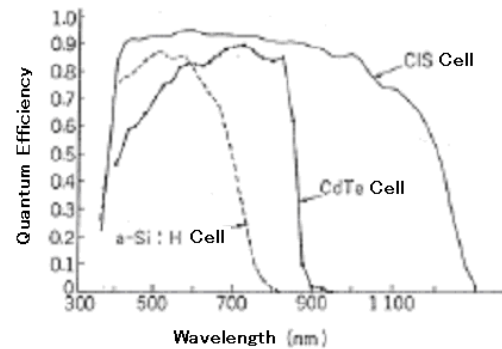
Fig. 2.3.9 Spectral sensitivities of solar cells 34
