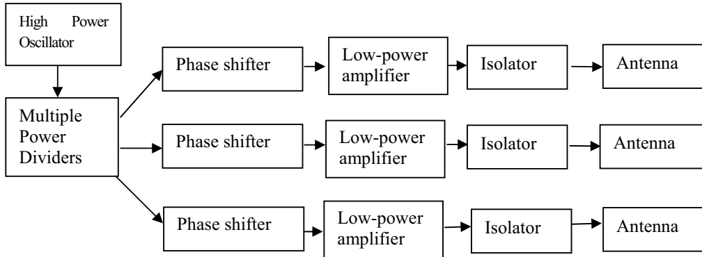
Fig. 2.3.14 Implementation of microwave transmission with phase shifters and low-power amplifiers for high-precision control of microwave beam direction without grating lobes 36
