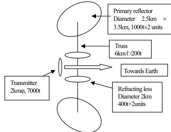
Fig. 2.4.7 Year 2002 Reference Model 89
