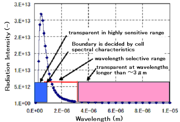
Figure 2.3.8 Effects of a spectral filter set between the sun and the solar cell 33
