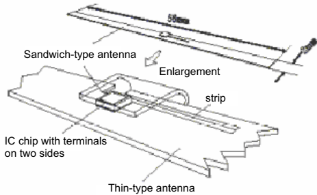
Fig. 3.6.2 μ-chip antenna 38
