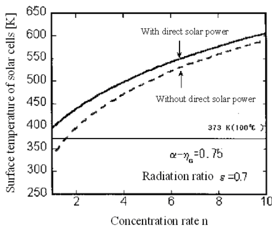
Fig. 2.3.7 Sun light concentration rate and balance temperature of generator ( \alpha absorption ratio of solar power; \eta_G , efficiency of solar cell) 32
