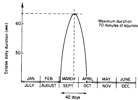
Fig. 2.1.2 Daily duration of eclipses as a function of the date. 2
